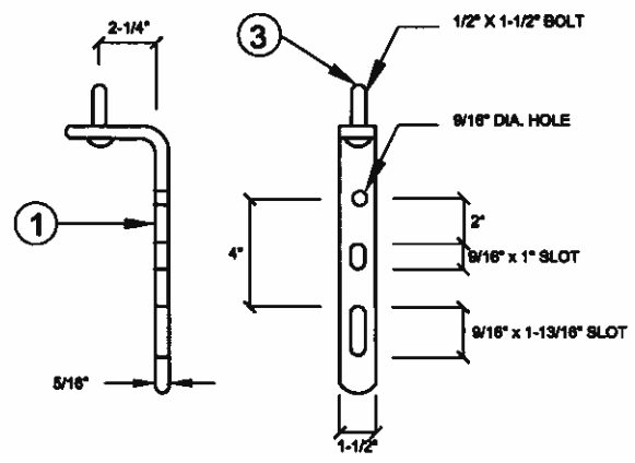
BRACKET DETAIL
